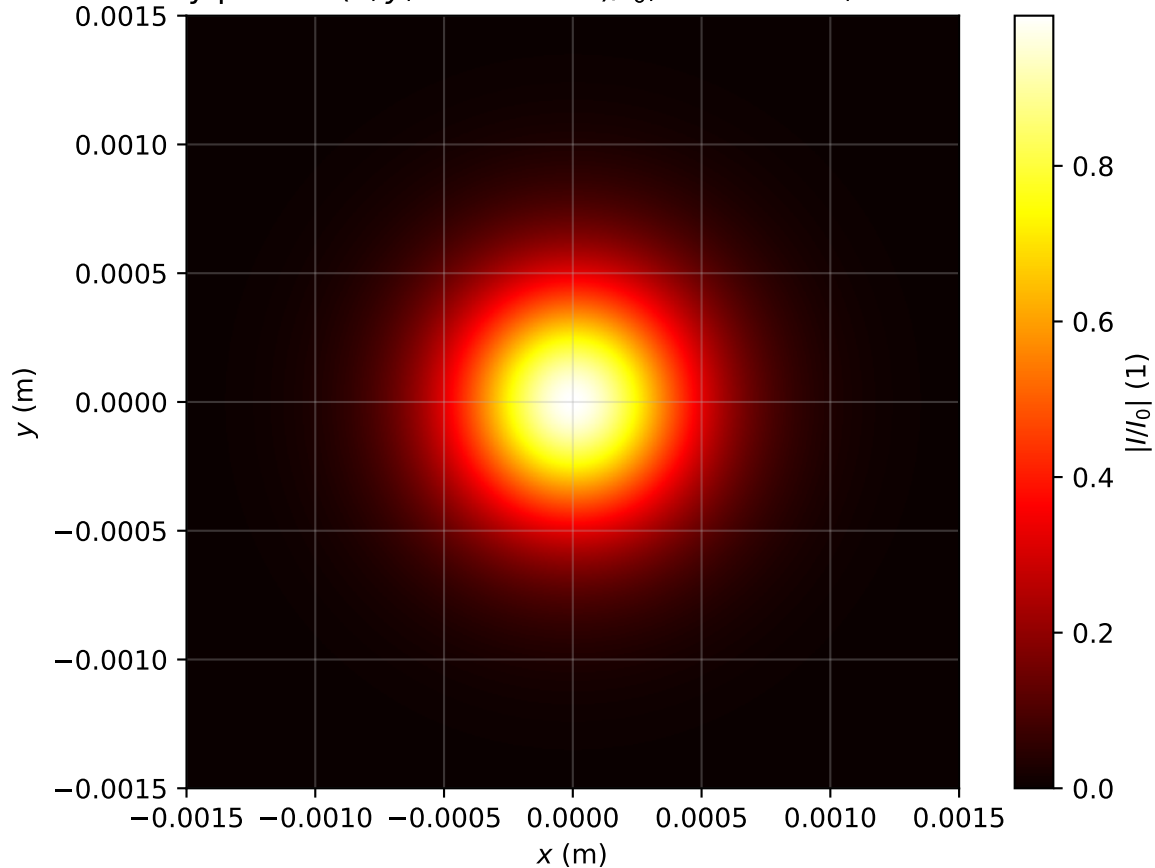
Intensity profile I(x, y, z = 1.353m)/I_0 , \text{Pin}=0.5\text{Pcr} , artificial time
